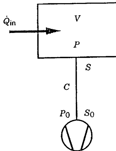
Fig. Schematic diagram - basic vacuum system
