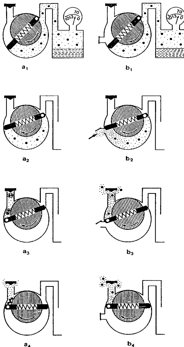
Fig. 13.1 Illustration of the pumping process in a rotary vane pump without (left) and with (right) gas ballast device when pumping condensable substances. ● vapour particles
