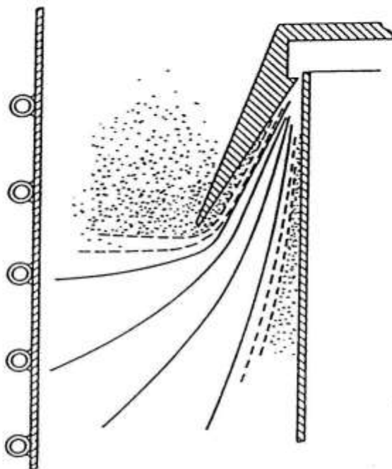
Fig. Representation of fluid jet emerging from a diffusion pump nozzle (Power & Crawley (1954))
